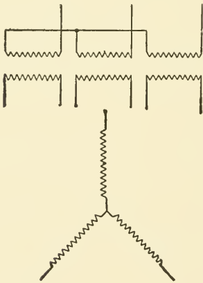
Fig. 29. Y Connections for Transformers
